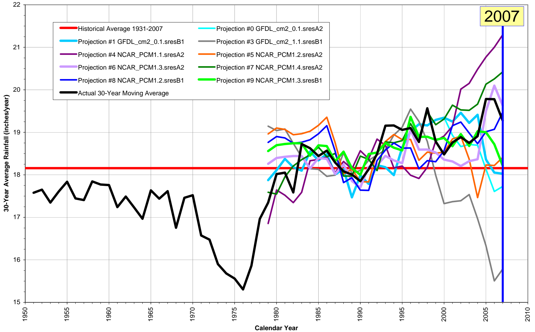
Figure D-1: 30-Year Moving Average Rainfall Projections at Newhall-Soledad Rain Gage (For Nine Studied Projections)
