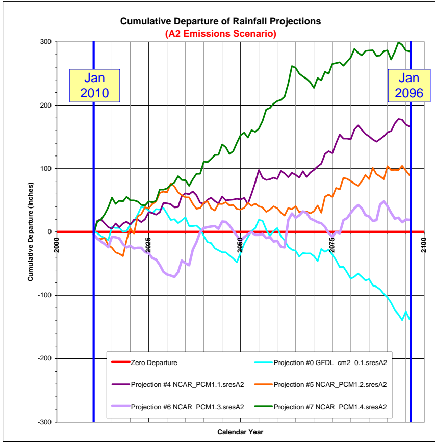
Figure D-8: Cumulative Departure from Average Annual Rainfall at Newhall-Soledad Rain Gage (2010-2095)
