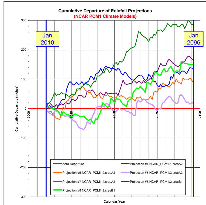
Figure D-6: Cumulative Departure from Average Annual Rainfall at Newhall-Soledad Rain Gage (2010-2095)
