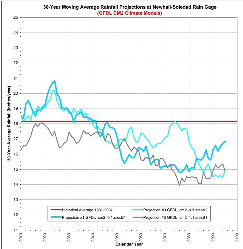
Figure D-5: 30-Year Moving Average Annual Rainfall at Newhall-Soledad Rain Gage (2010 - 2095)
