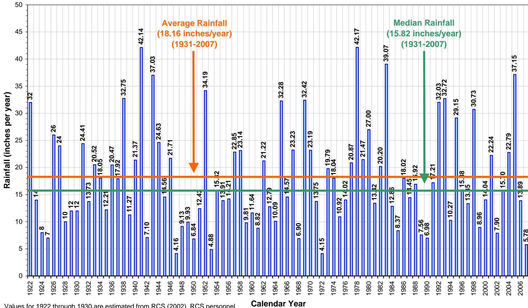
Figure 3-1 Annual Rainfall (Newhall-Soledad Rain Gage)
