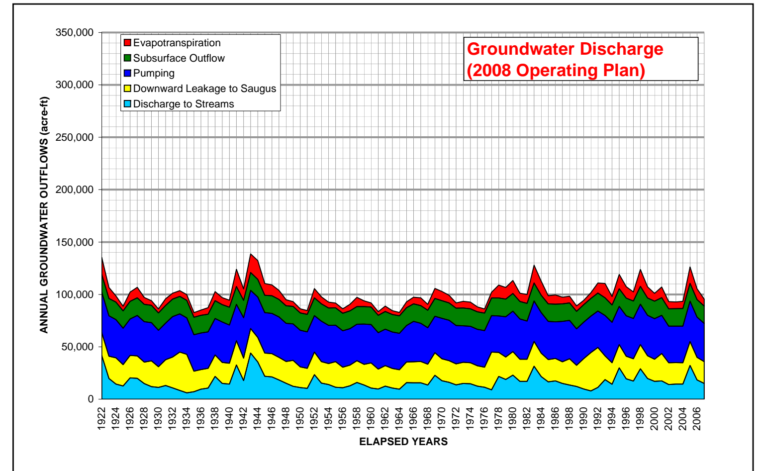
Figure 4-16: Comparison of Simulated Trends in Groundwater Recharge and Discharge Terms for the 2008 Operating Plan Under Historical Hydrology
