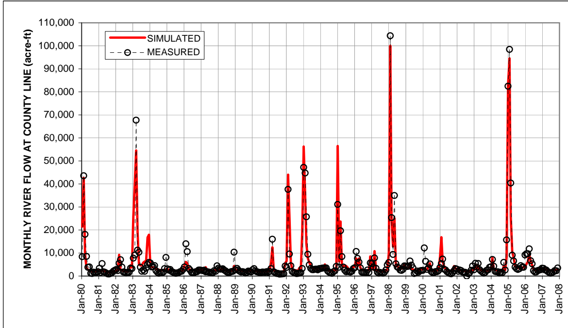
Modeled and Measured Monthly Flow in the Santa Clara River at the County Line
