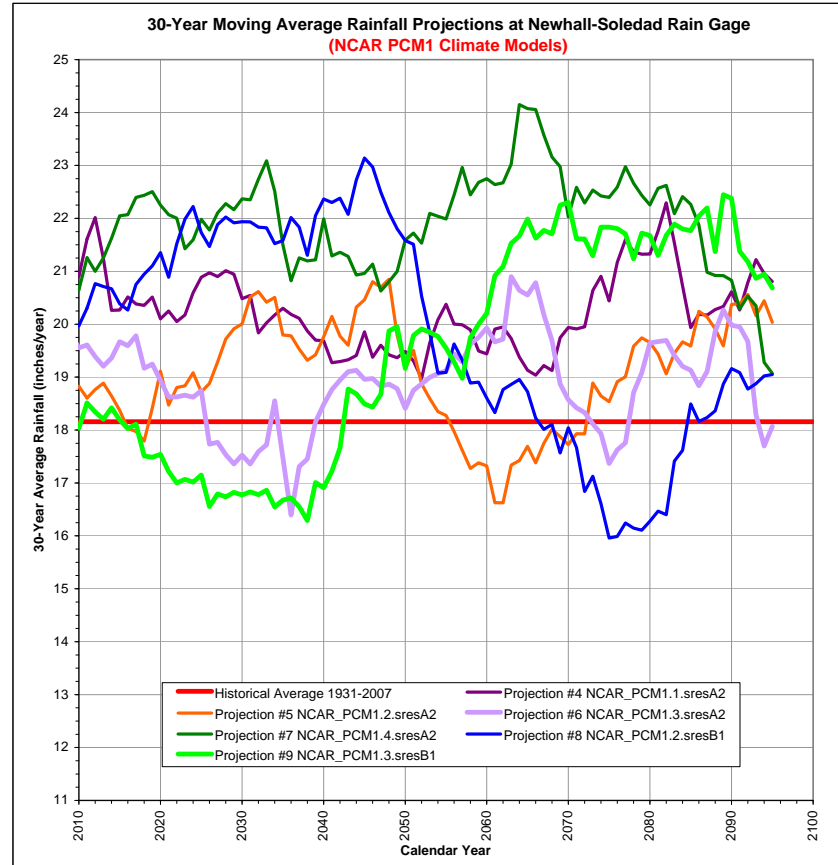
Figure D-5: 30-Year Moving Average Annual Rainfall at Newhall-Soledad Rain Gage (2010 - 2095)
