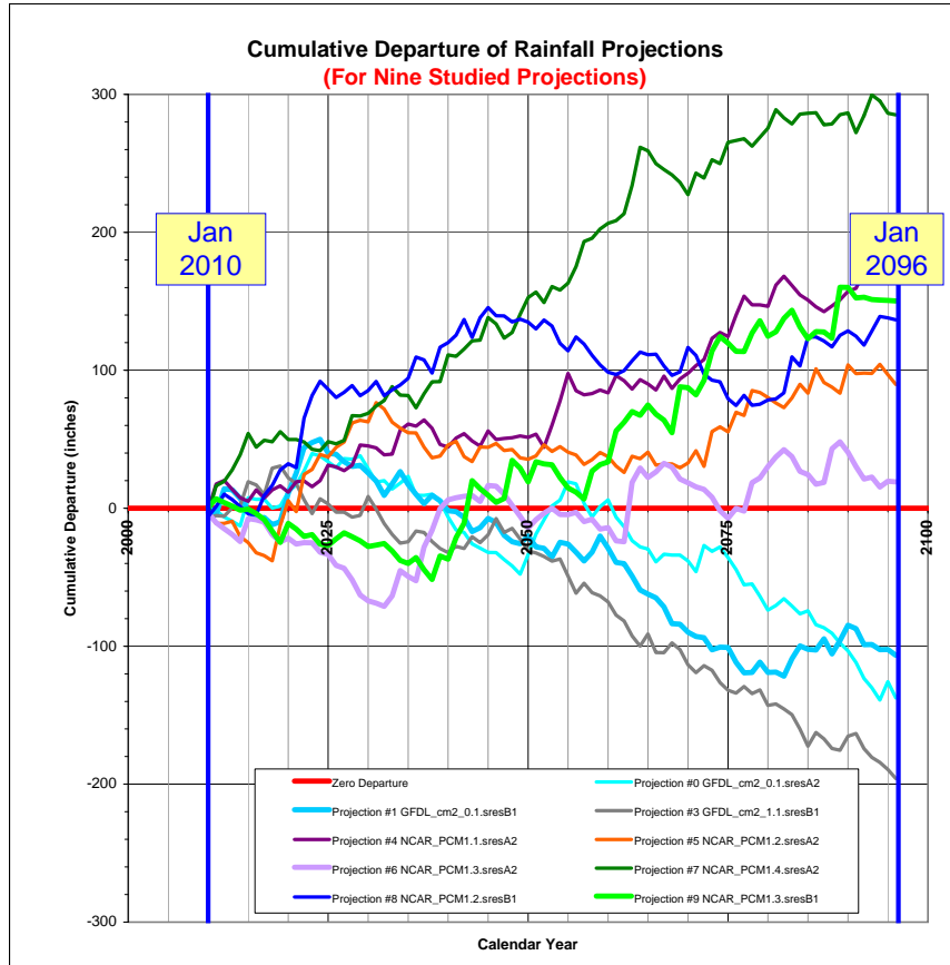
Figure D-4: Cumulative Departure from Average Annual Rainfall at Newhall-Soledad Rain Gage (2010-2095)
