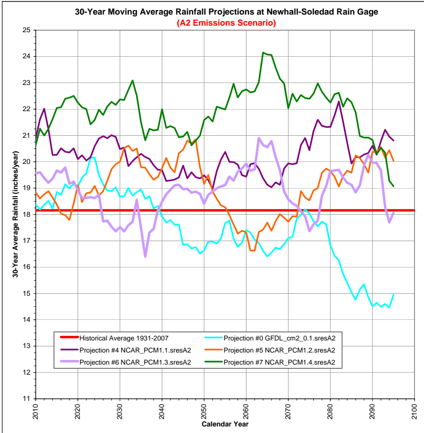
Figure D-7: 30-Year Moving Average Annual Rainfall at Newhall-Soledad Rain Gage (2010 - 2095)
