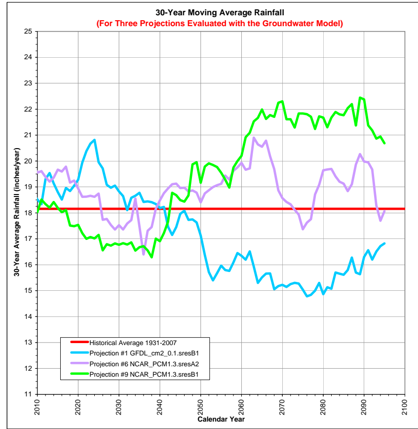
Figure D-3: 30-Year Moving Average Annual Rainfall at Newhall-Soledad Rain Gage (2010 - 2095)
