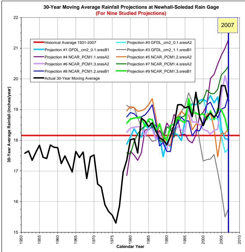
Figure D-2: 30-Year Moving Average Annual Rainfall at Newhall-Soledad Rain Gage (1950 - 2007)
