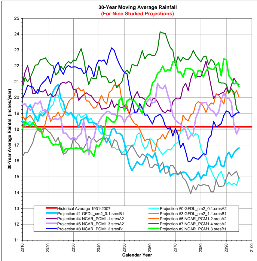
Figure D-3: 30-Year Moving Average Annual Rainfall at Newhall-Soledad Rain Gage (2010 - 2095)
