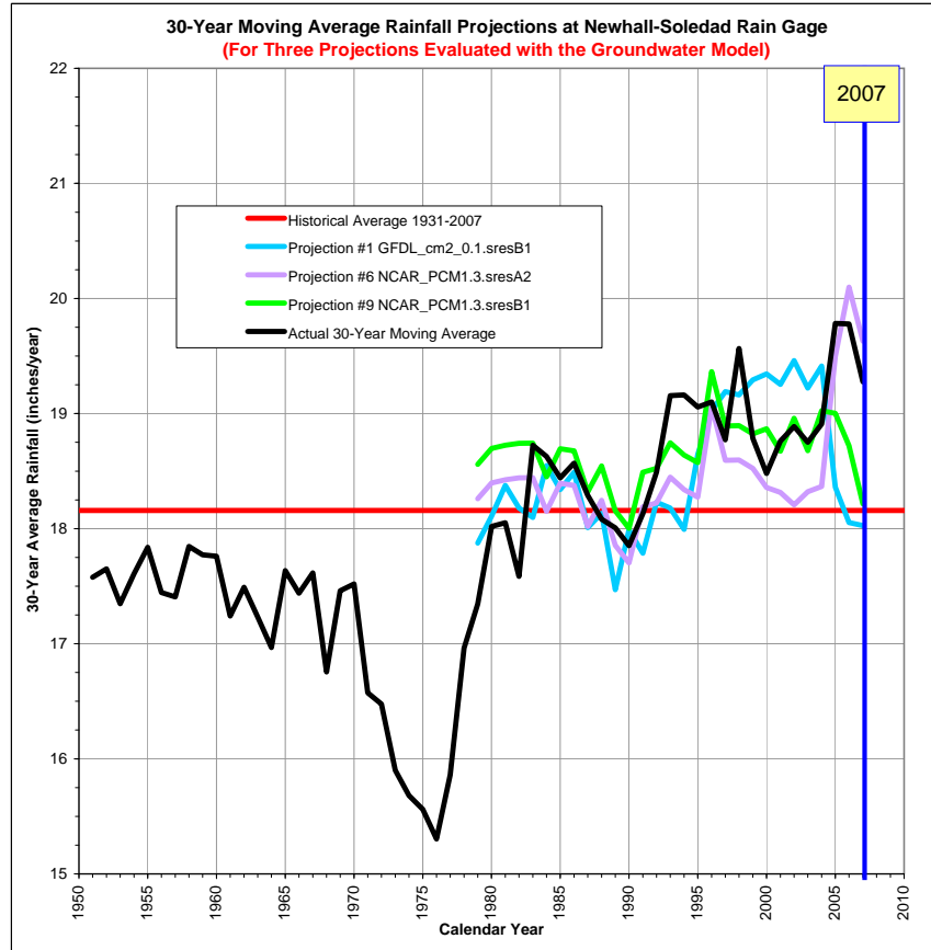
Figure D-2: 30-Year Moving Average Annual Rainfall at Newhall-Soledad Rain Gage (1950 - 2007)
